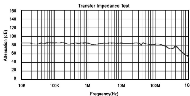
Shielding performance
